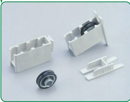
ROLLER R-750 AND TANDEM ROLLER T-750
