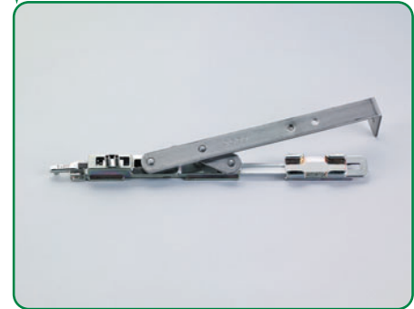
SHORT ARM B-2051 TILT FIRST OPENING
