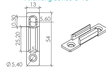
Cerradero marco C-13 Frame Striker C-13
