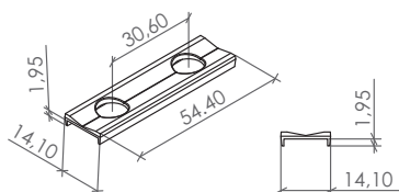
Calce C-14 Frame Striker Adaptor C-14
