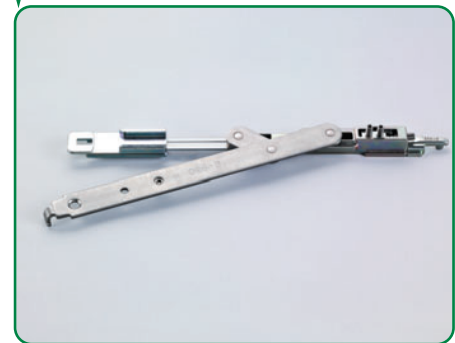
SHORT ARM B-6011 TRADITIONAL OPENING
